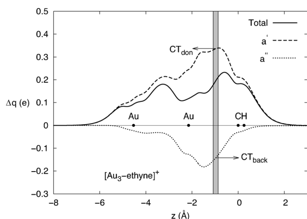
Figure 1. Charge displacement functions for the complex [\text{Au}_3\text{-ethyne}]^+ . The dots on the axis mark the z coordinate of the atoms. The vertical band marks the isodensity boundary between the \text{Au}_3^+ and ethyne fragments (see text for details).
